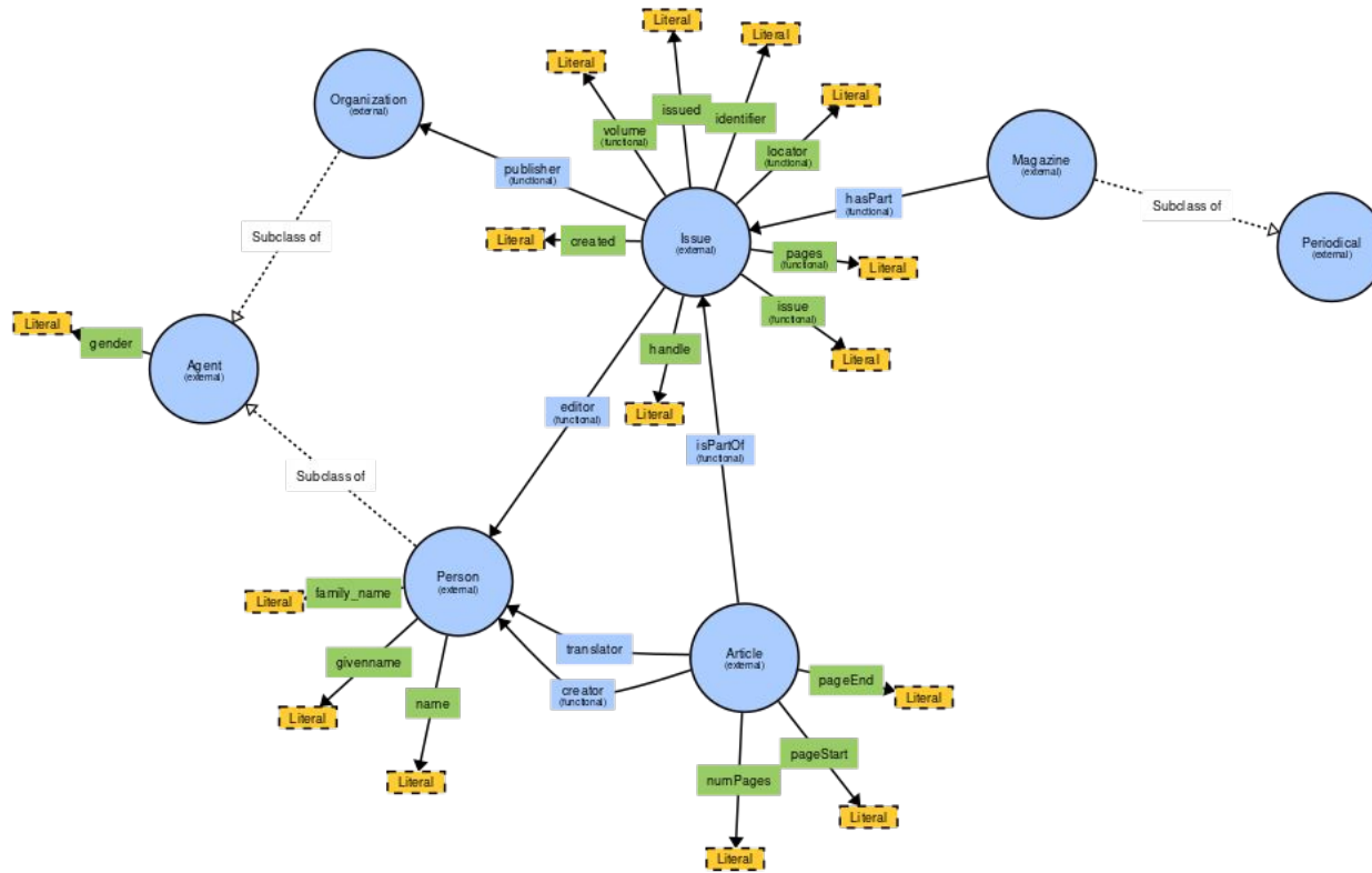
Example of Data Model (Ontology)
